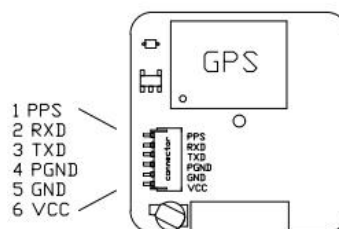
Figure 2: Pin Assignment
