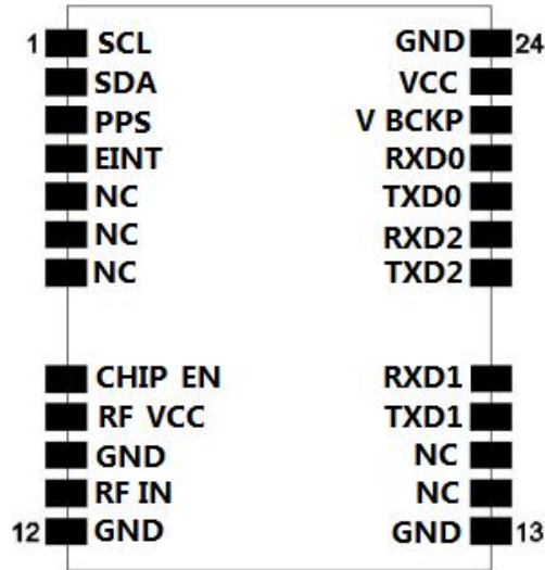
Figure3: Pin Assignment
