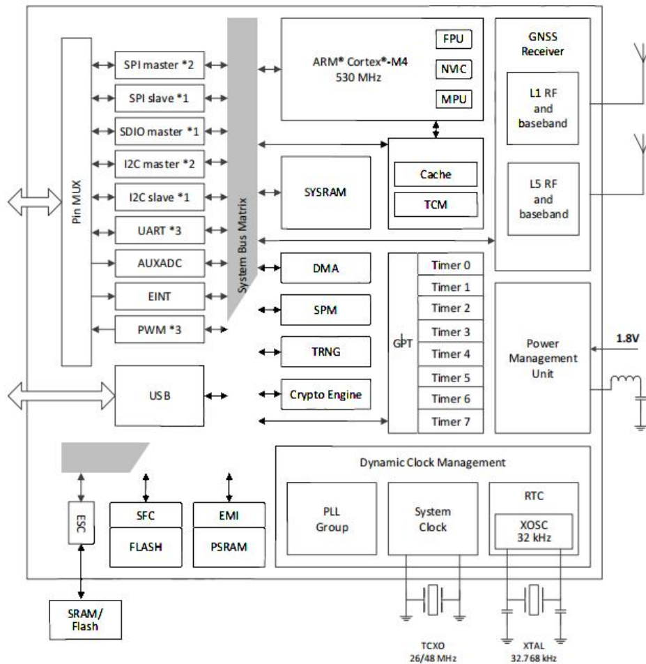
Figure 1-2 : Block Diagram
