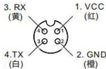
Figure 2: Pin Assignment
