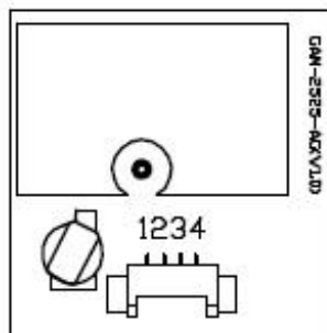
Figure 2: Pin Assignment
