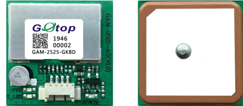
Figure : GAM-2525-GKBD Top View
