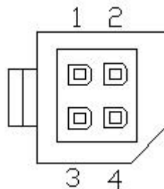
Figure 2: Pin Assignment
